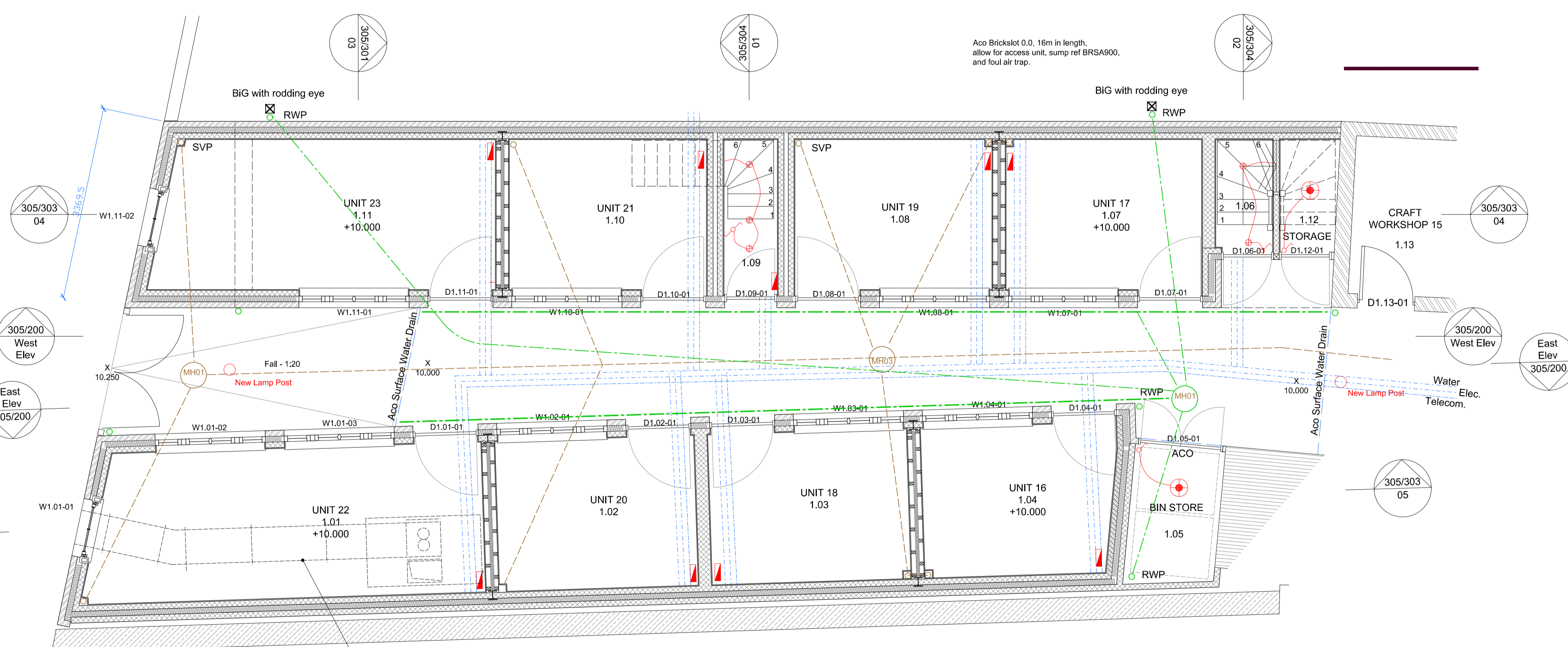
GROUND FLOOR
